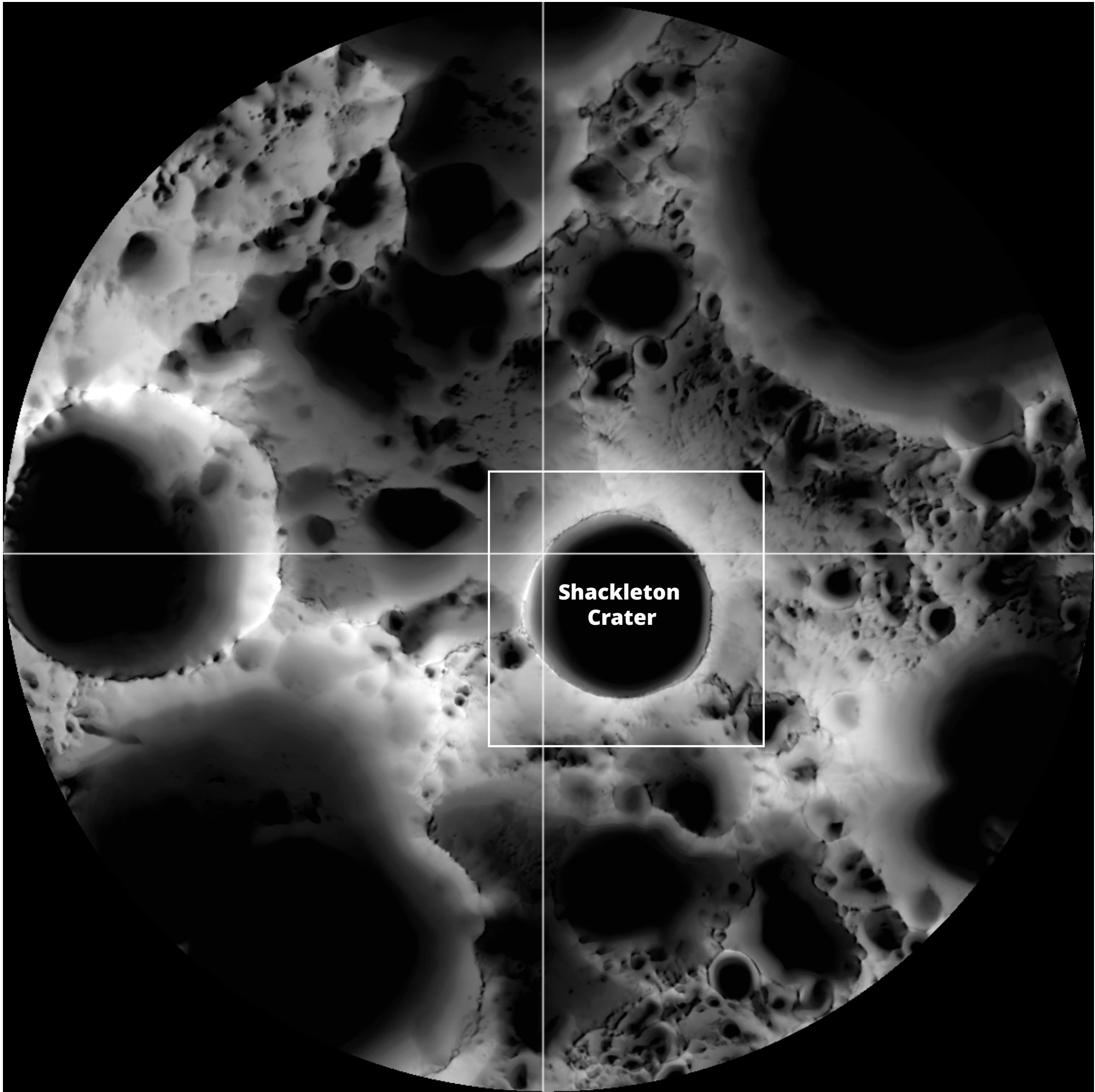
Lunar illuminated days LUNAR RECONNAISSANCE ORBITER: Permanently Shadowed Regions on the Moon 2010 www.nasa.gov
